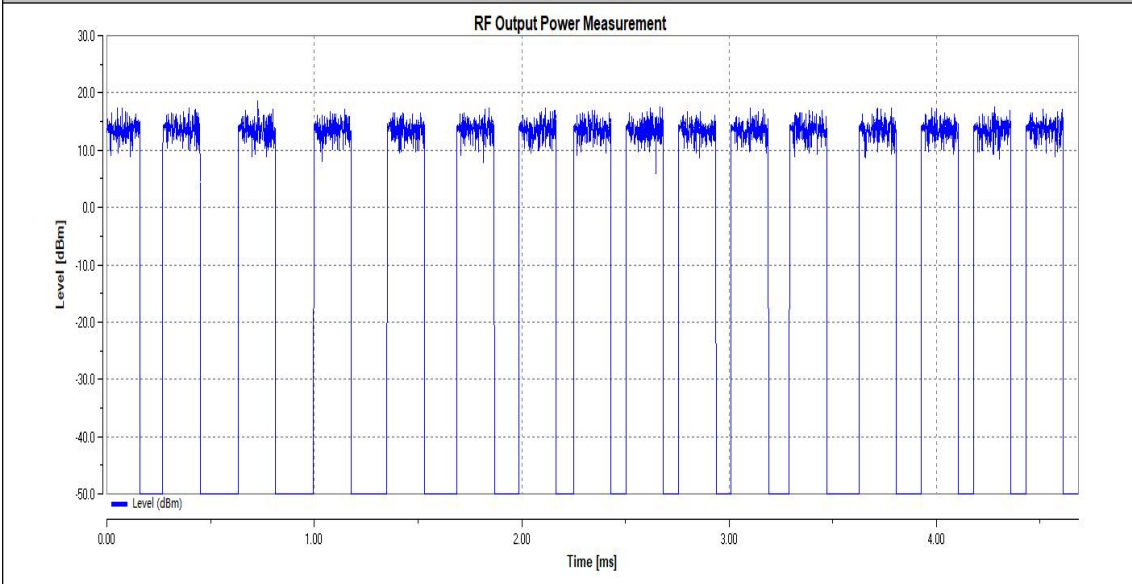
HTNV_11G_Ant1_2442
