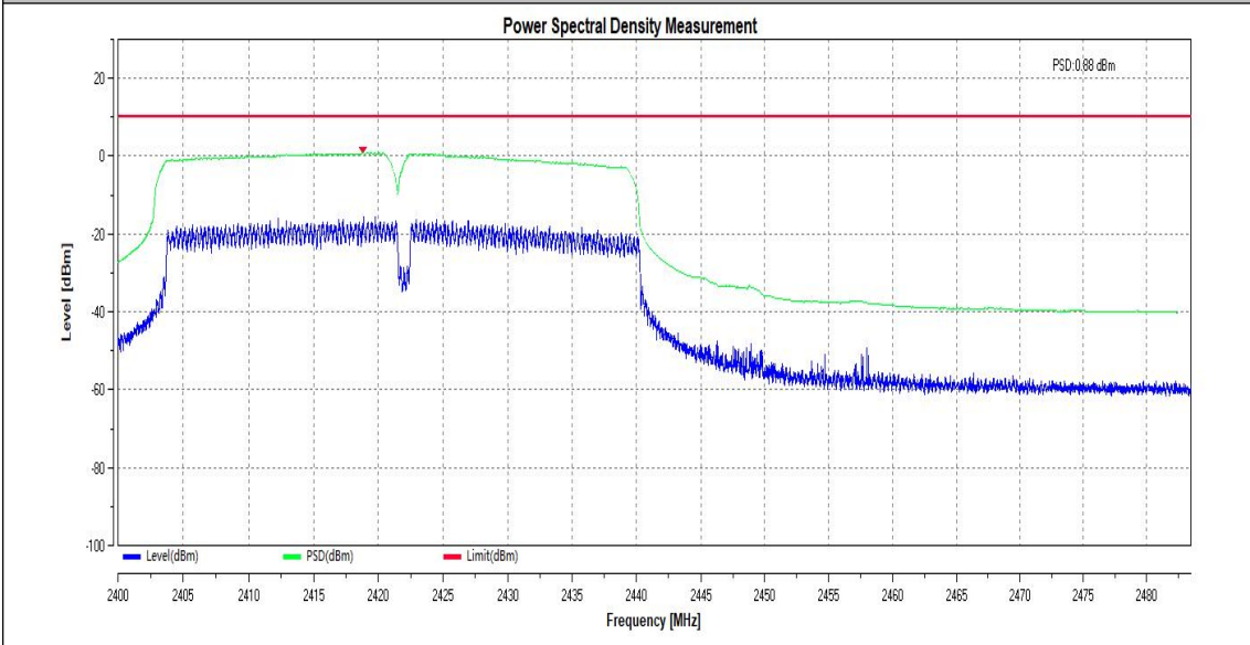
11N40SISO_Ant1_2442
