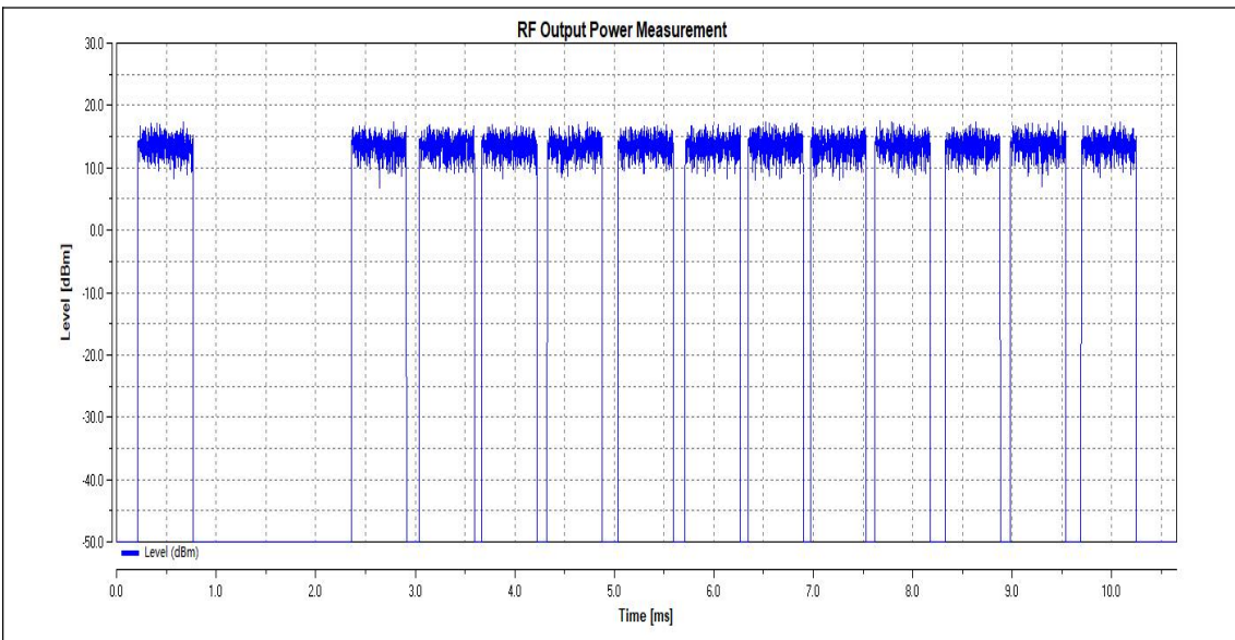
HTNV_11N20SISO_Ant1_2442
