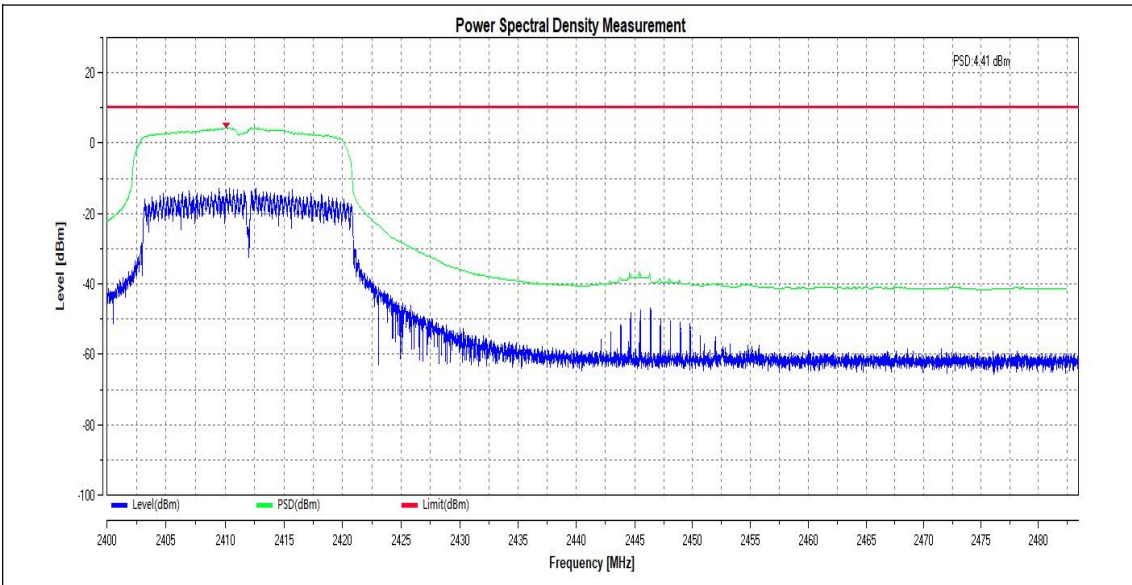
11N20SISO_Ant1_2442
