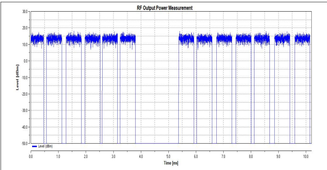
LTNV_11N20SISO_Ant1_2442
