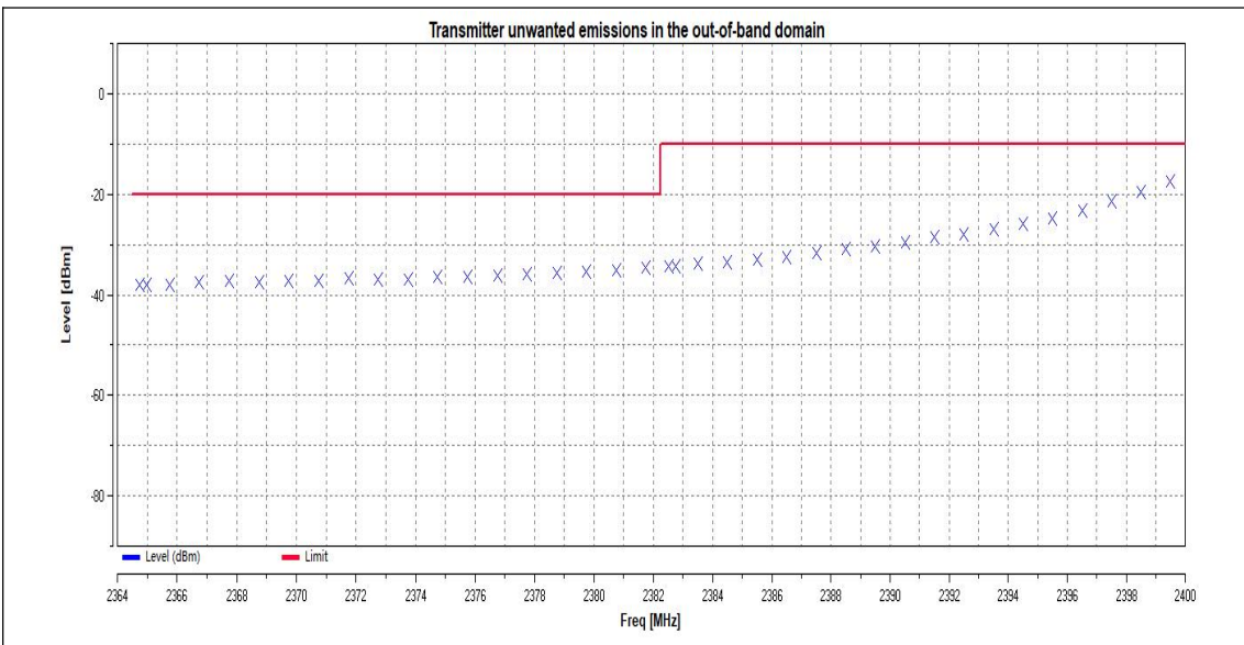
11N20SISO_Ant1_2472_2483.5MHz to 2483.5MHz+2BW
