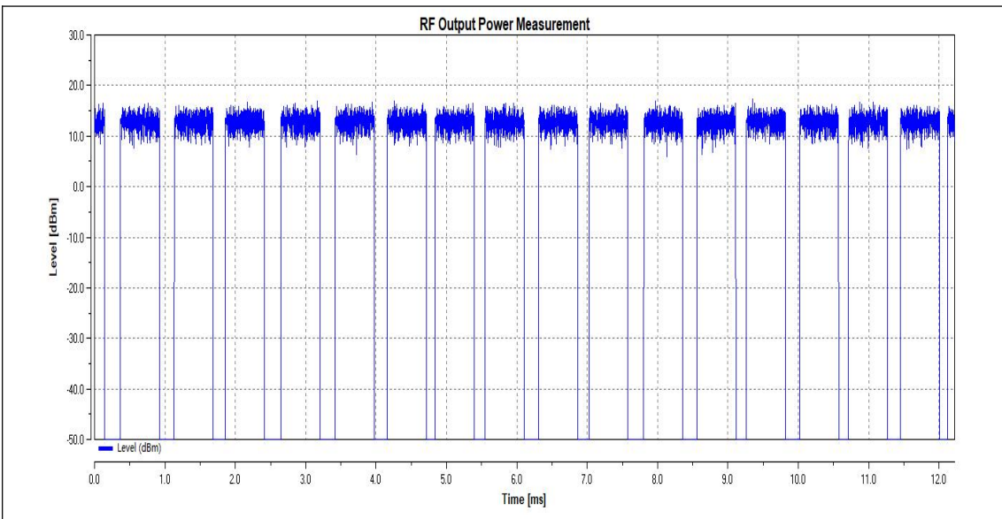
NTVN_11N40SISO_Ant1_2422
