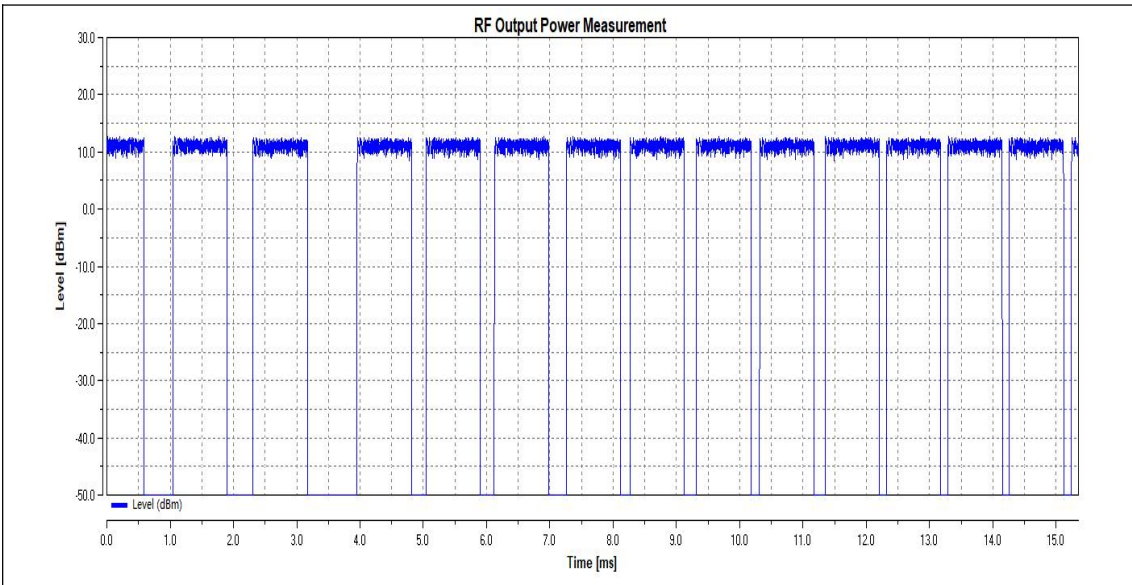
HTNV_11G_Ant1_2412
