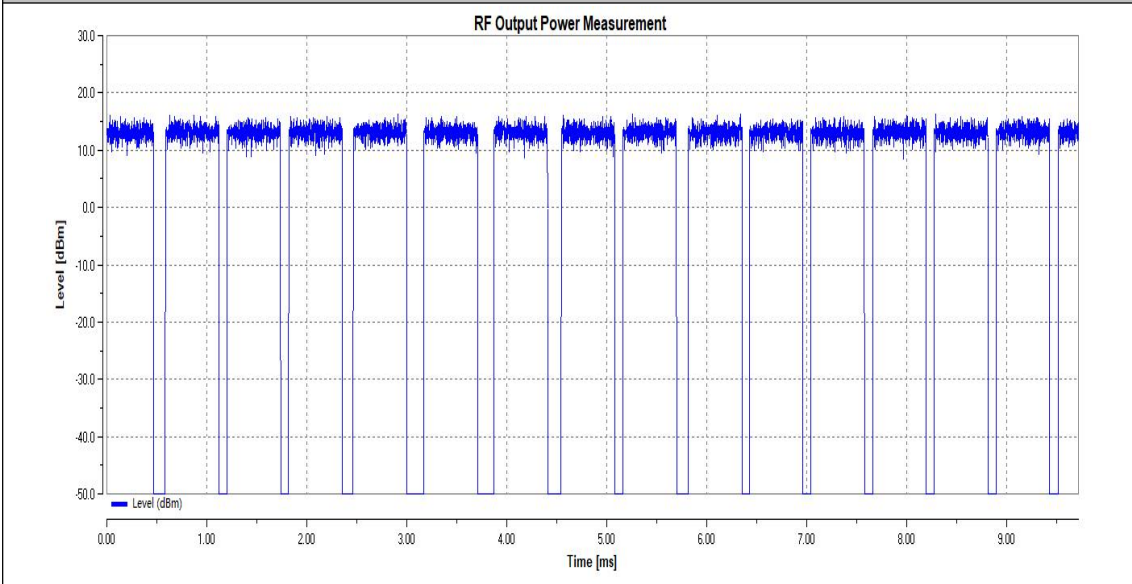
LTNV_11N40SISO_Ant1_2422
