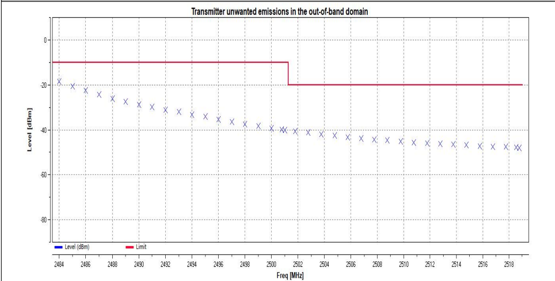
11N40SISO_Ant1_2422_2400MHz-2BW to 2400MHz
