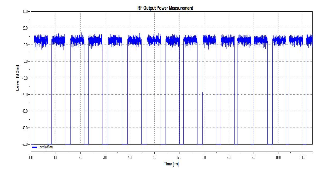
HTNV_11N40SISO_Ant1_2422
