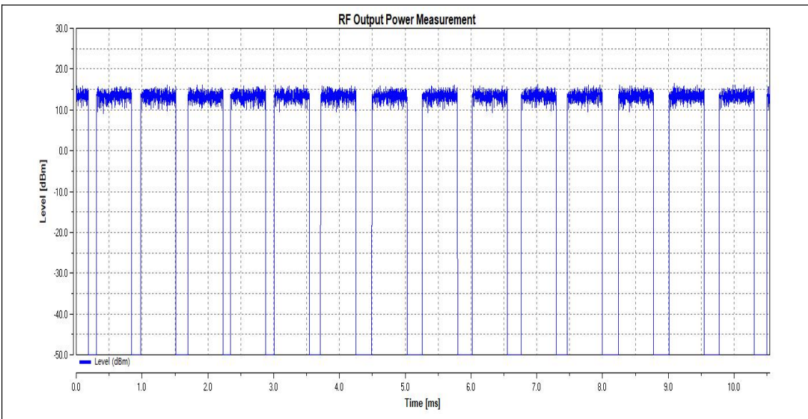
NTNV_11N40SISO_Ant1_2462
