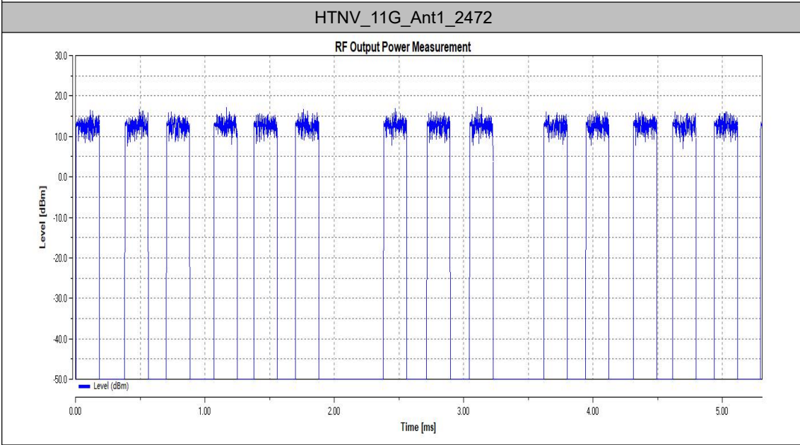
HTNV_11N20SISO_Ant1_2412
