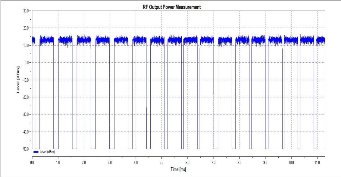
HTNV_11N40SISO_Ant1_2442
