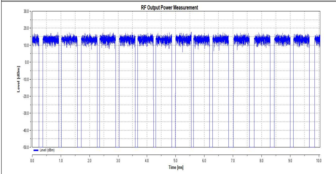
NTNV_11N20SISO_Ant1_2472
