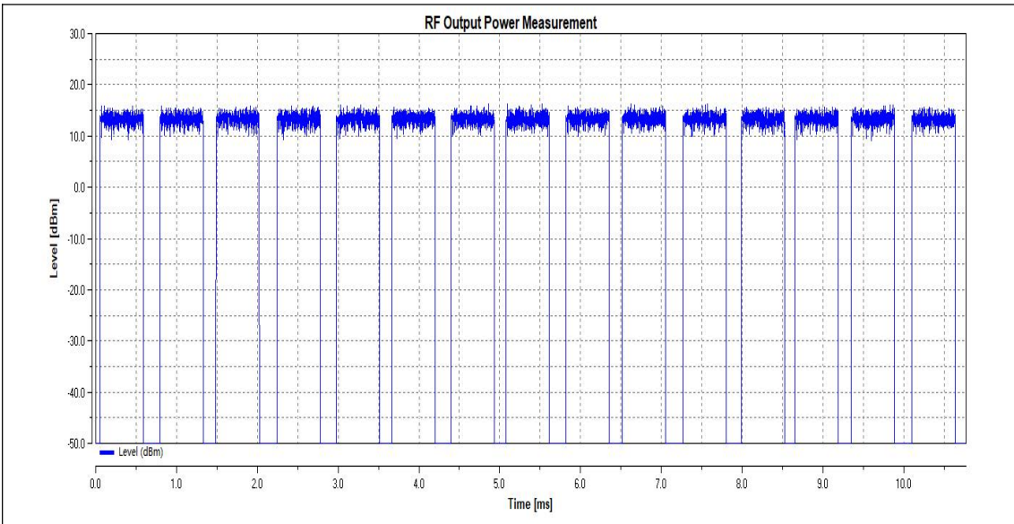
HTNV_11N40SISO_Ant1_2462
