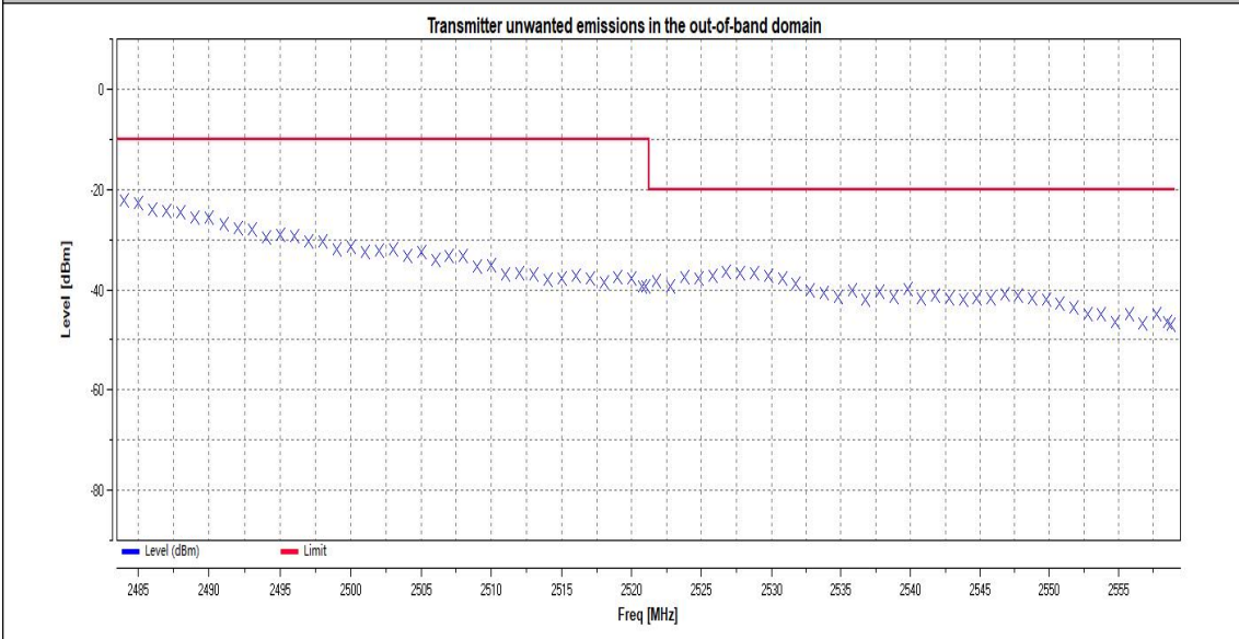
11AX40SISO_Ant1_2462_2483.5MHz to 2483.5MHz+2BW
