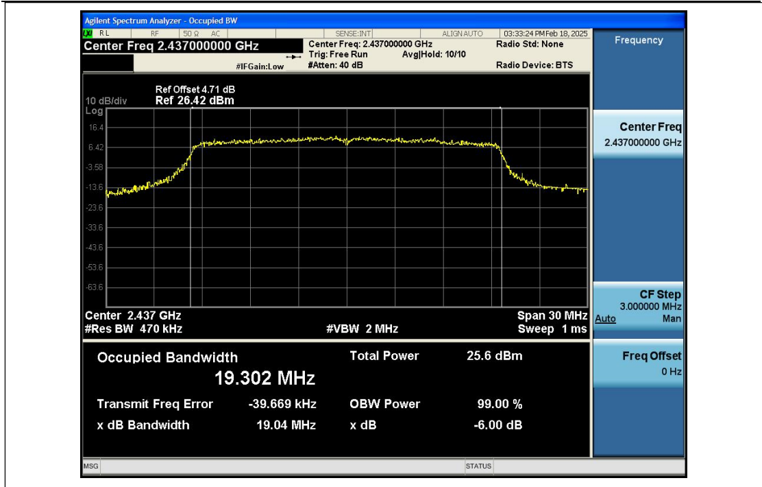
-6dB_Bandwidth_NVNT_ANT1_802_11ax(HEW20)_2462
