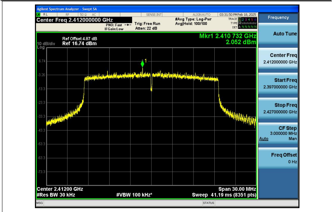
Power_Spectral_Density_NVNT_ANT1_802_11ax(HEW20)_2437
