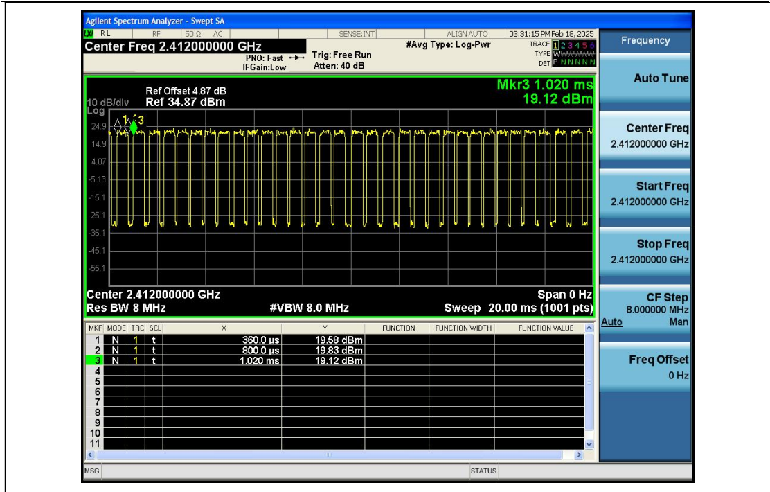
Duty_Cycle_NVNT_ANT1_802_11ax(HEW20)_2437
