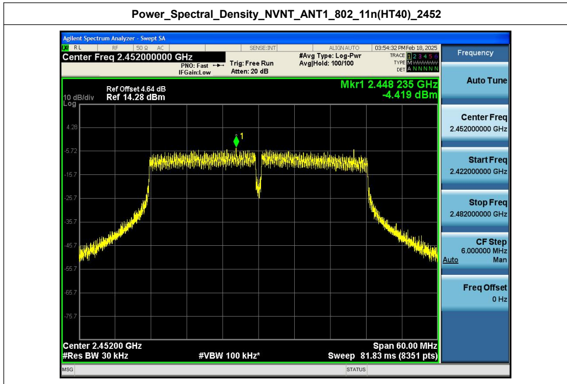
Power_Spectral_Density_NVNT_ANT1_802_11x(HEW40)_2422
