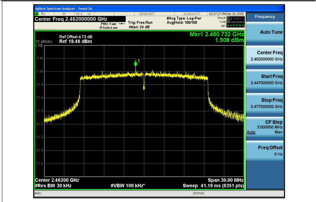
Power_Spectral_Density_NVNT_ANT1_802_11n(HT40)_2422
