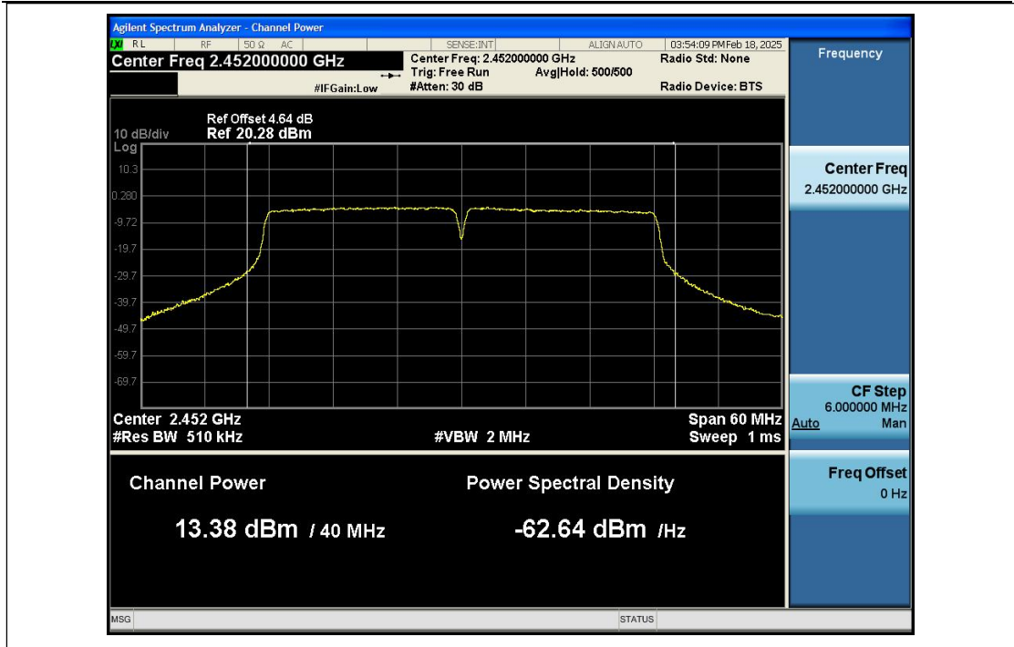
MAX__Output_Power_NVNT_ANT1_802_11ax(HEW40)_2422
