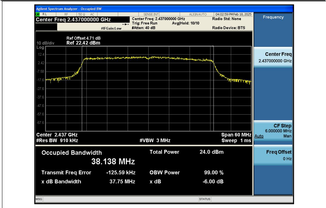
-6dB_Bandwidth_NVNT_ANT1_802_11ax(HEW40)_2452
