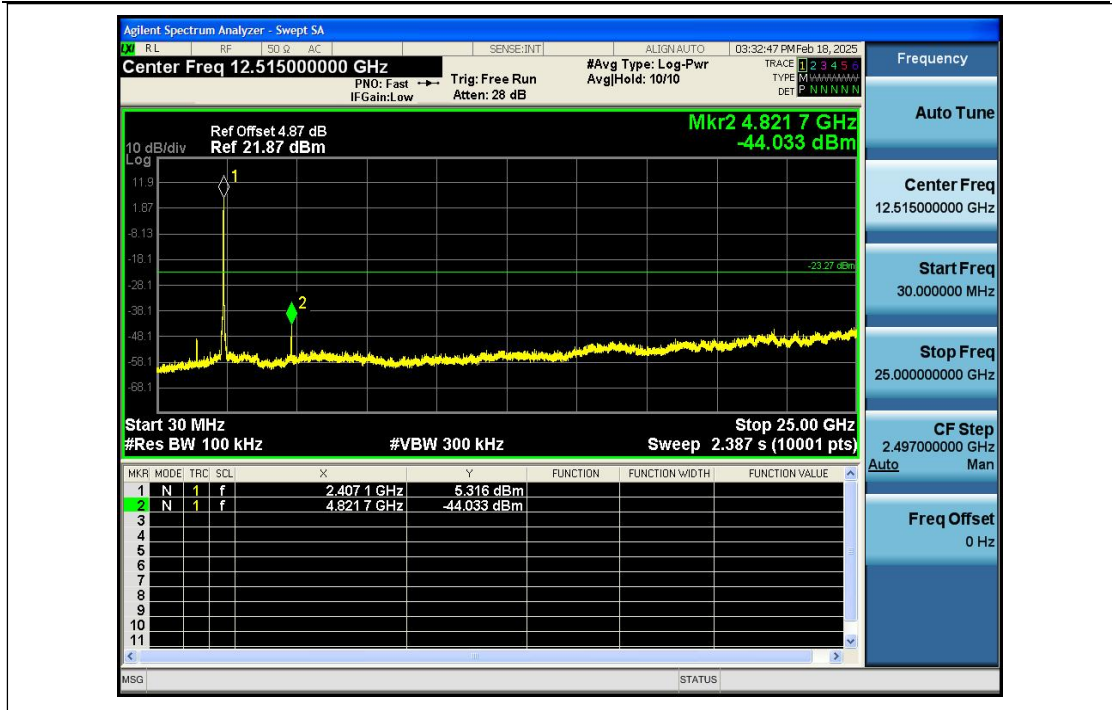
1_Reference_Level_NVNT_ANT1_802_11ax(HEW20)_2437
