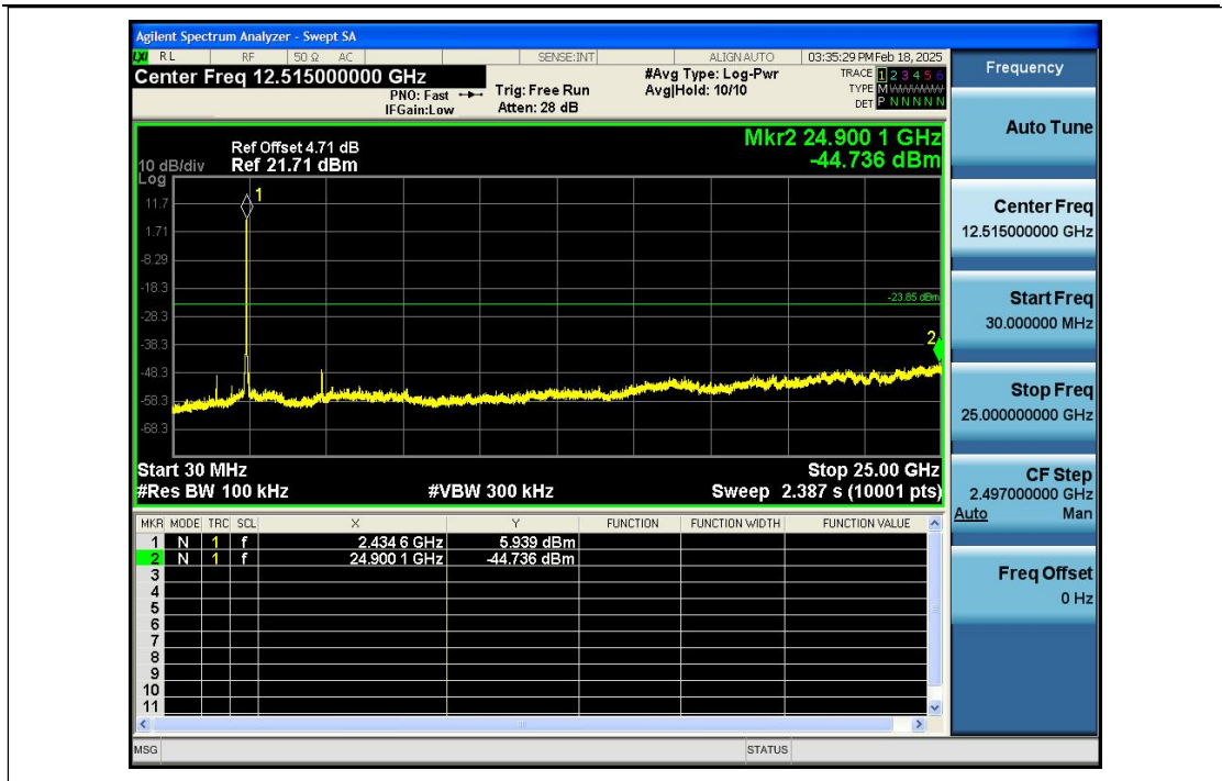
1_Reference_Level_NVNT_ANT1_802_11ax(HEW20)_2462
