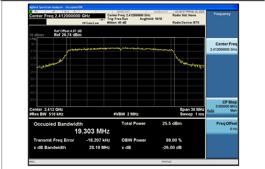
99%_Occupied_Bandwidth_NVNT_ANT1_802_11ax(HEW20)_2437
