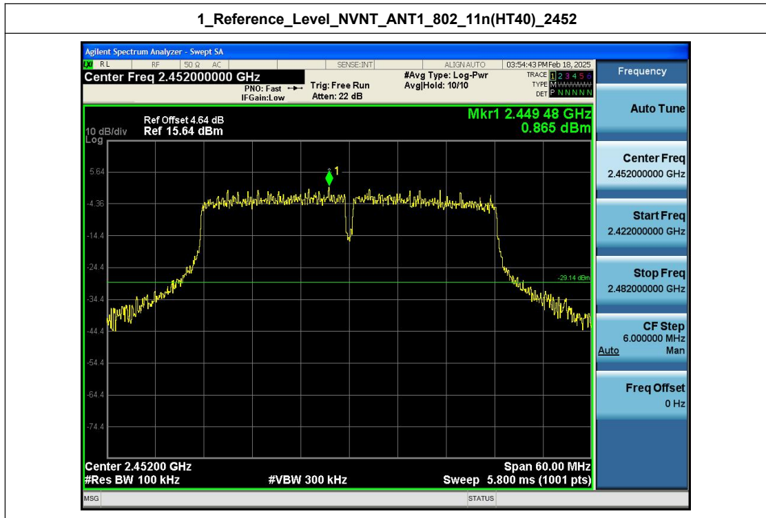
2_Spurious_Emission_NVNT_ANT1_802_11n(HT40)_2452
