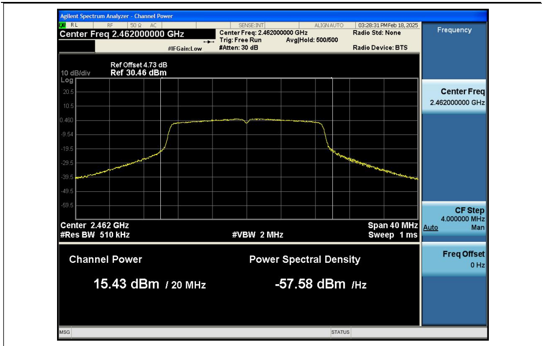
MAX__Output_Power_NVNT_ANT1_802_11ax(HEW20)_2412
