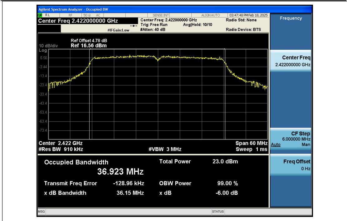
-6dB_Bandwidth_NVNT_ANT1_802_11n(HT40)_2437
