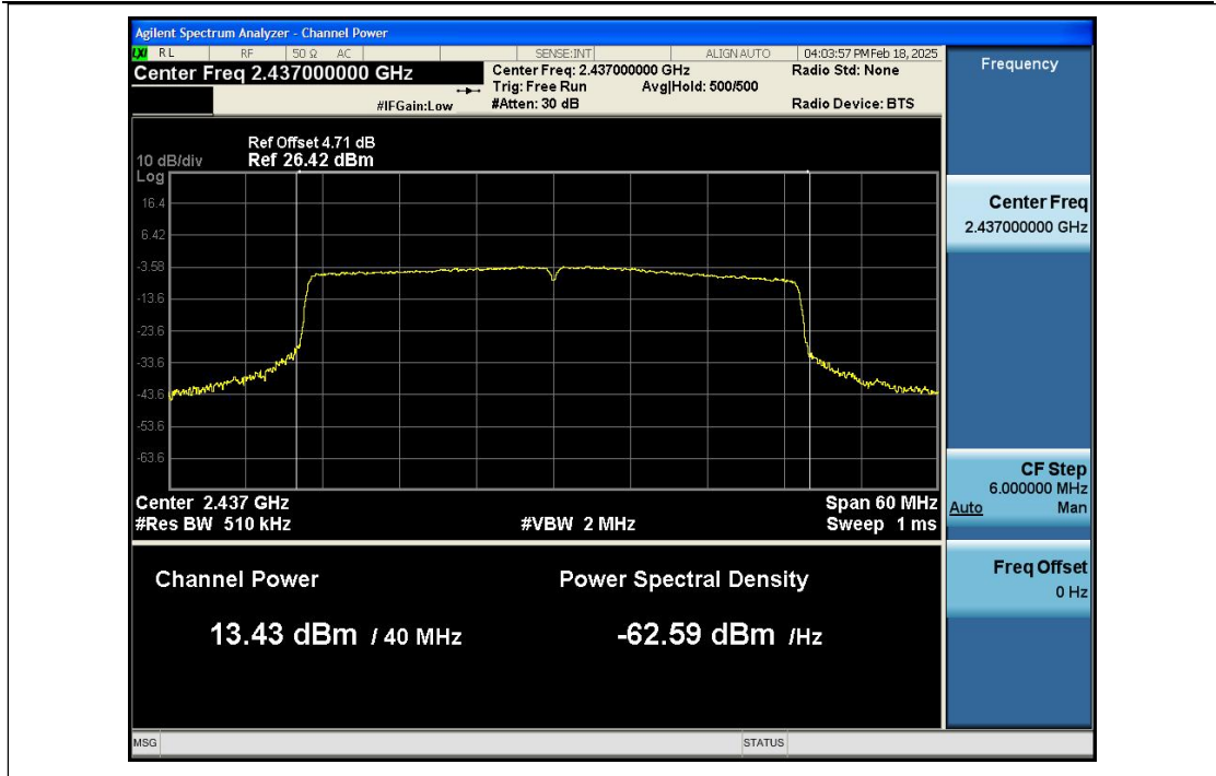
MAX__Output_Power_NVNT_ANT1_802_11ax(HEW40)_2452
