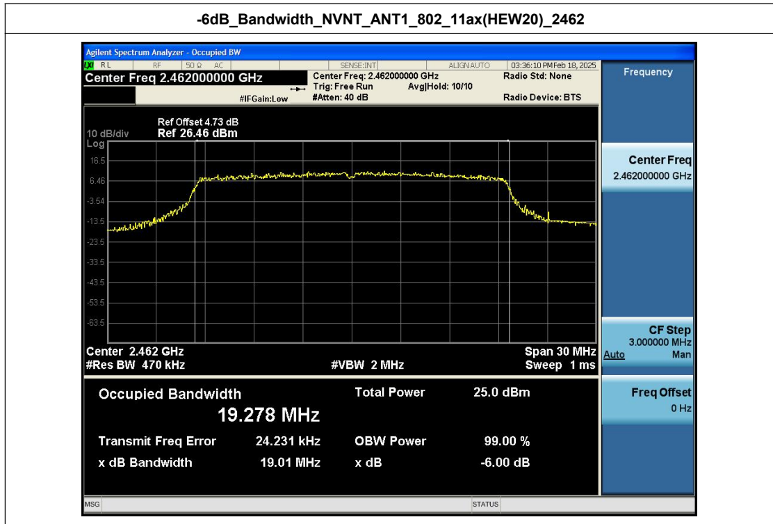
-6dB_Bandwidth_NVNT_ANT1_802_11n(HT40)_2422
