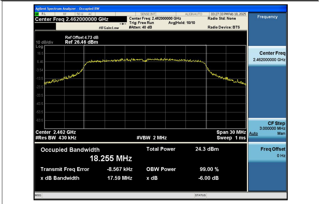
-6dB_Bandwidth_NVNT_ANT1_802_11ax(HEW20)_2412
