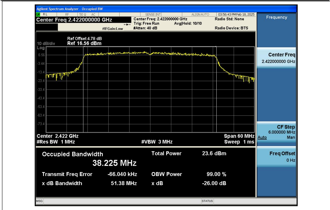
99%_Occupied_Bandwidth_NVNT_ANT1_802_11ax(HEW40)_2437
