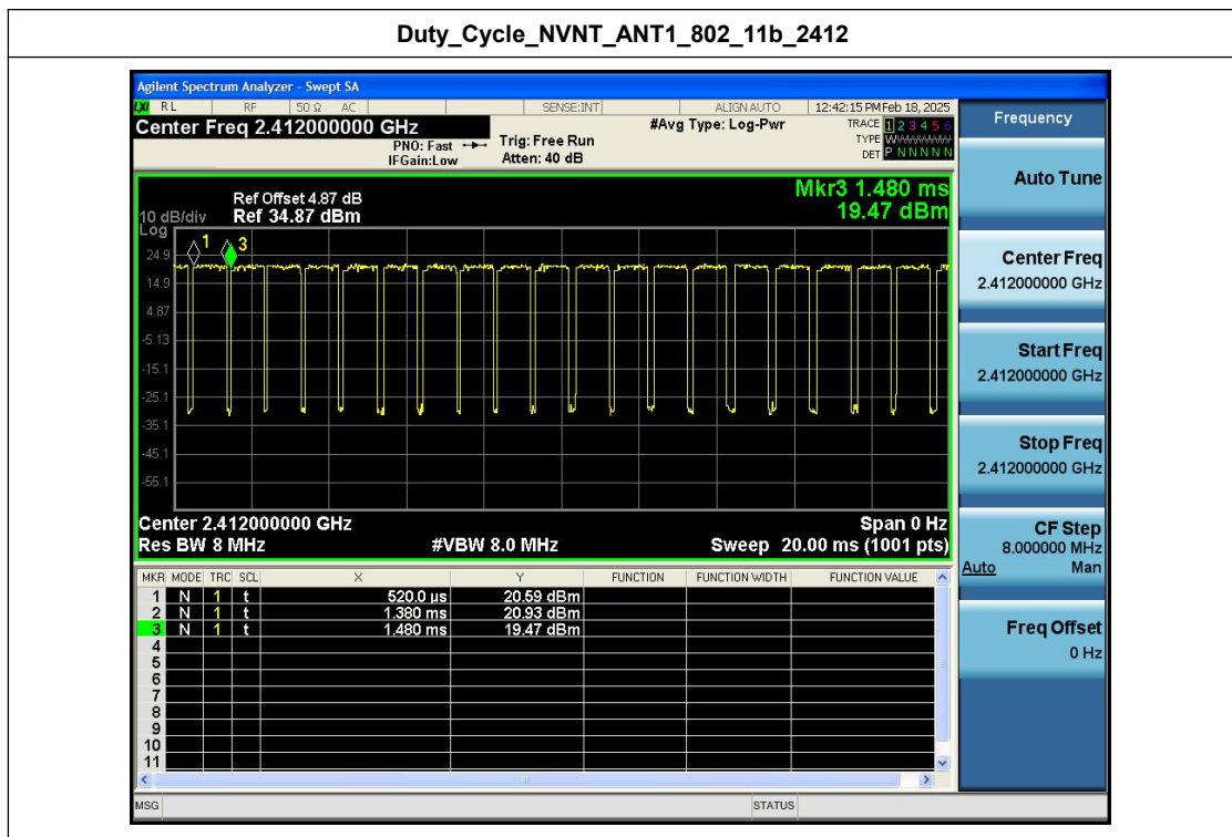
Duty_Cycle_NVNT_ANT1_802_11b_2437
