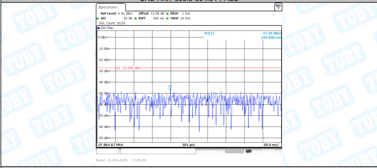
SRD-Ant1-865.5-864.67-PASS
