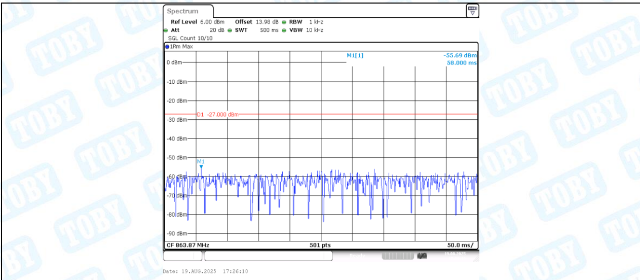
SRD-Ant1-863.5-863.87-PASS
