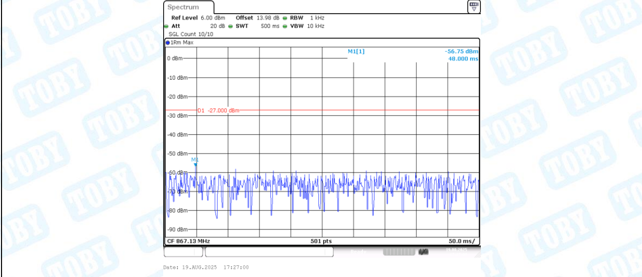
SRD-Ant1-865.5-867.13-PASS
